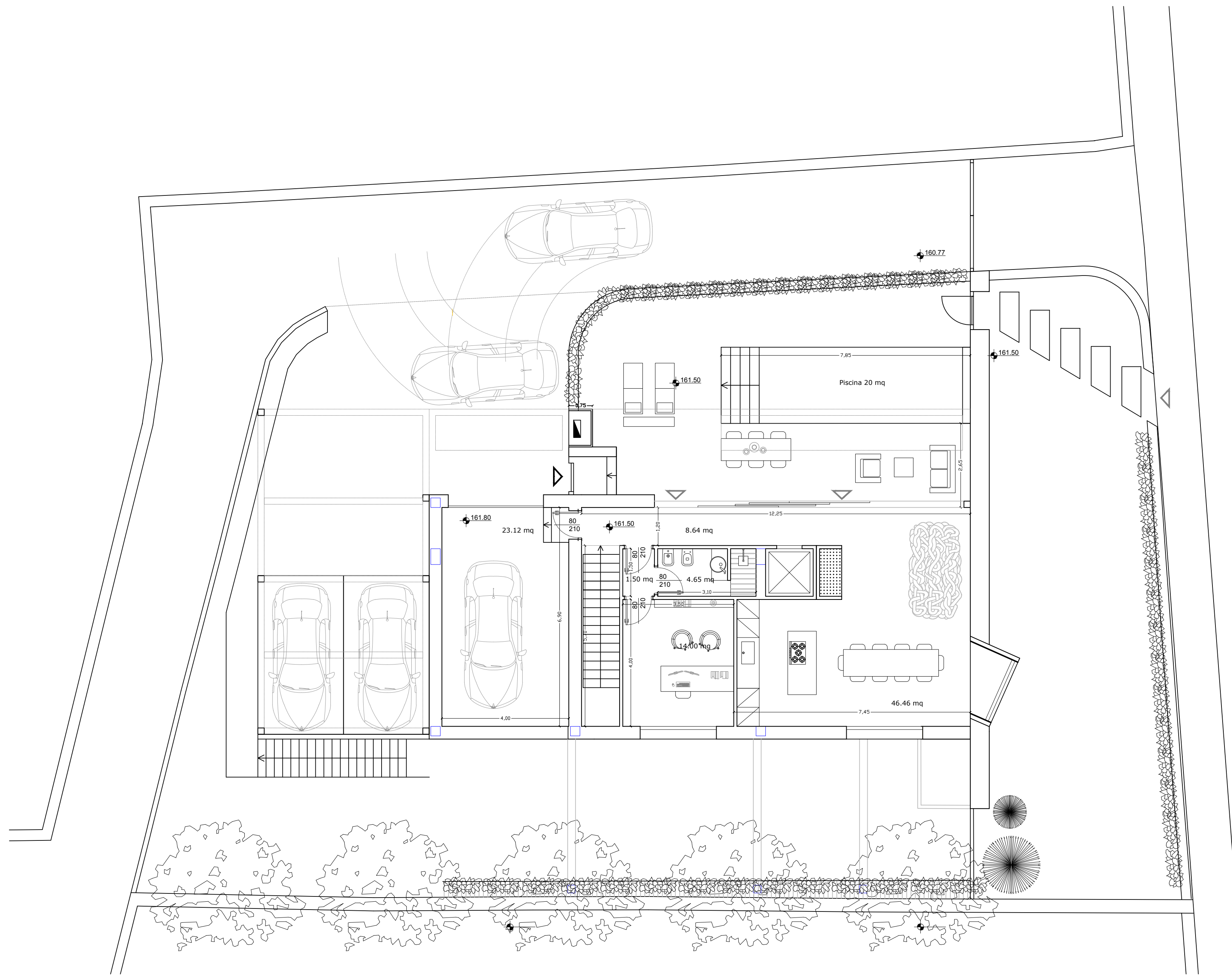
Planimetria piano terra
